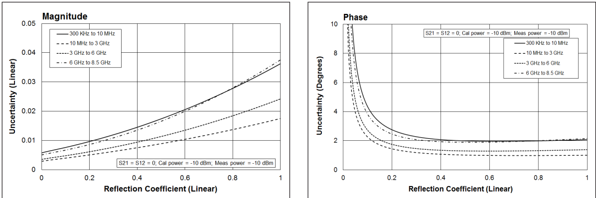
Reflection uncertainty (specification)
