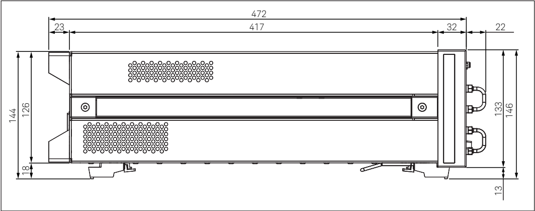
Figure 13. Dimensions (side view, with Option E5092A-020, in millimeters, nominal)
