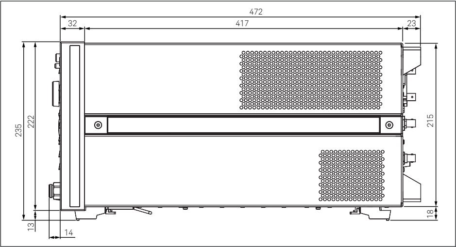
Figure 9. Dimensions (side view, E5071C with Option 2D5/2K5/4D5/4K5, in millimeters)
