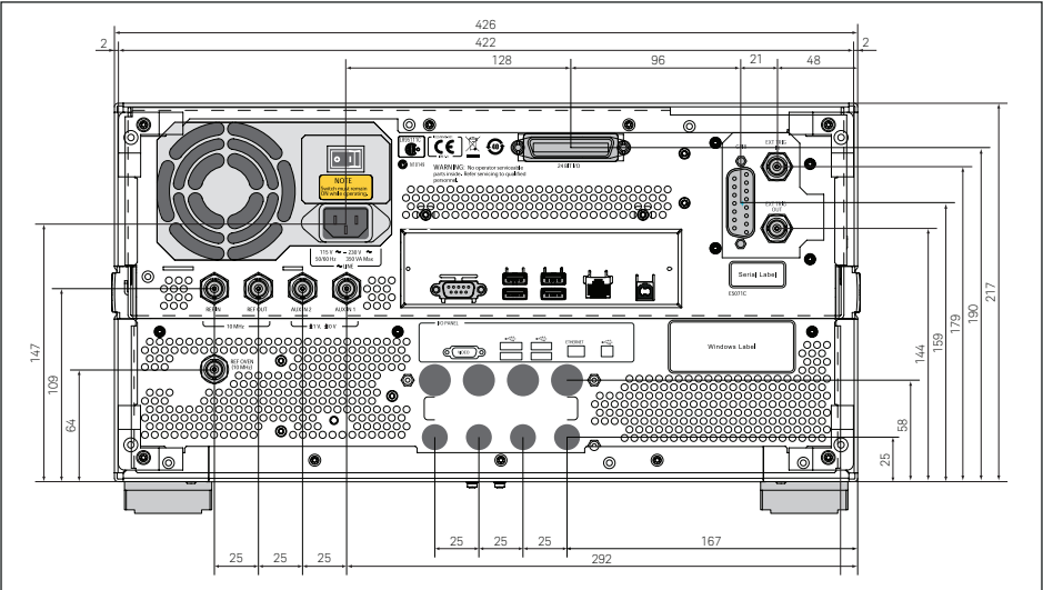
Figure 7. Dimensions (rear view with Option 1E5, in millimeters)
