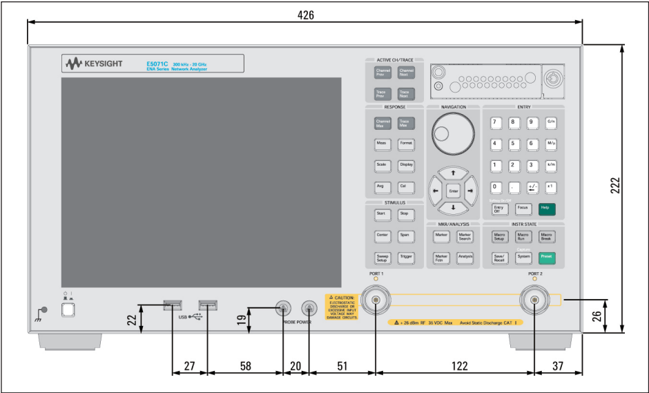
Figure 5. Dimensions (front view, E5071C with Option 2D5/2K5, in millimeters)
