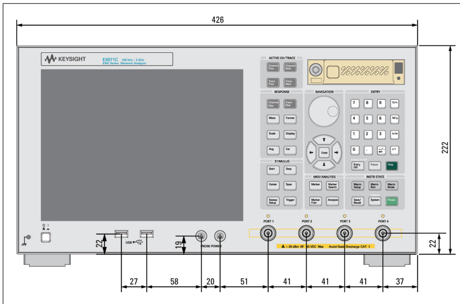
Figure 4. Dimensions (front view, E5071C with Option 430/435/440/445/460/465/480/485, in millimeters)
