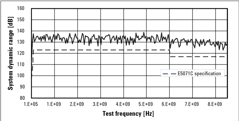
Figure 1. System dynamic range (specification and actual measurement data example, IF bandwidth 10 Hz)
