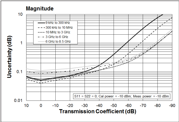
Transmission uncertainty (specification)
