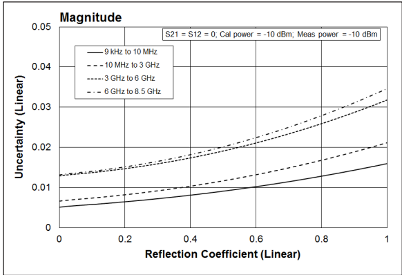
Reflection uncertainty (specification)
